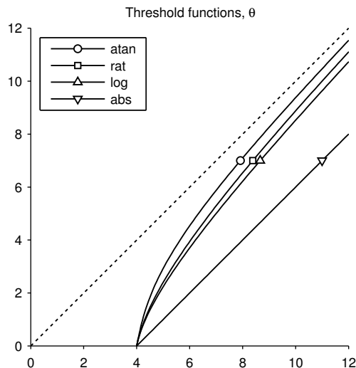
Fig. 2. Threshold functions derived from the four penalty functions given in Sec. II-B; three of which are non-convex.
