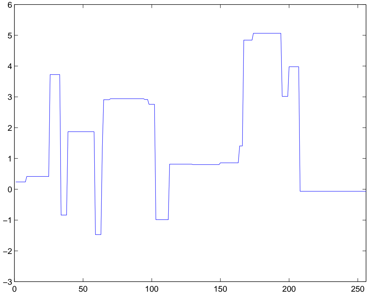
TV denoising using MCP penalty
