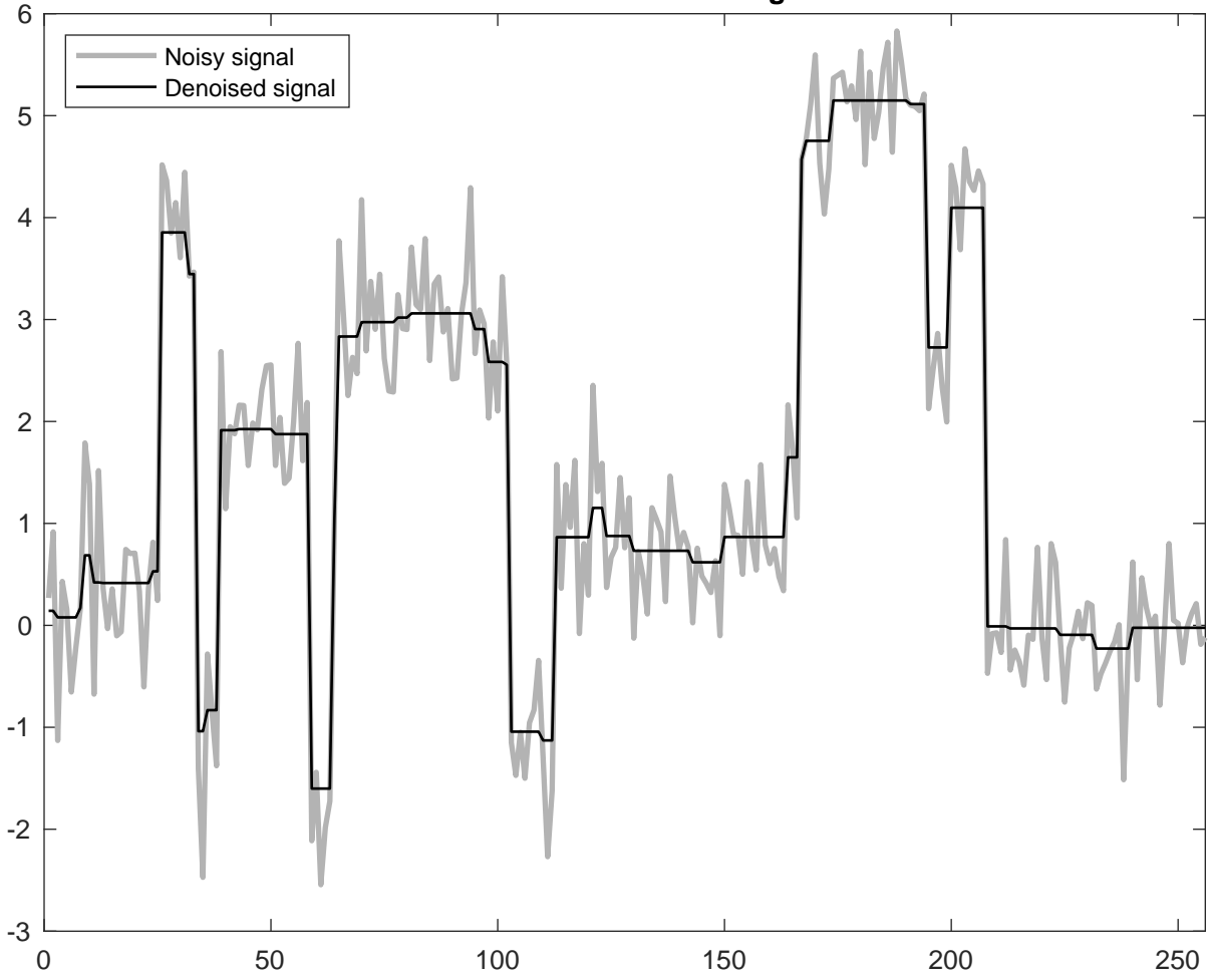
Classical TV denoising
