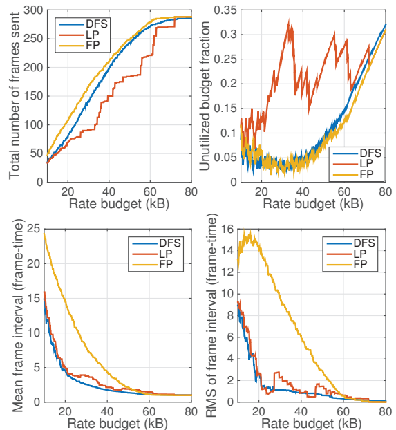
Figure 4: Comparison of DFS with FP and LP; number of frames sent (upper-left), unused budget (upper-right), mean and standard deviation of the frame intervals (lower-left and lower-right). Encoding frame rate is 30 Hz, thus frame-time is 1/30 sec.
